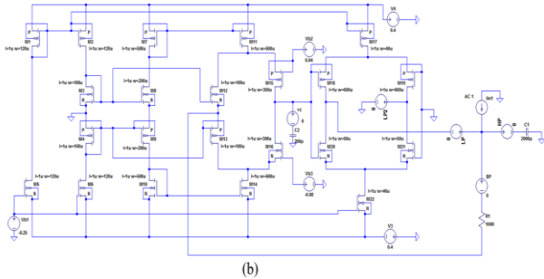
Figure 6. (a) CDTA Filter Circuit (b) Implemented Filter Circuit via LTSPICE Program
