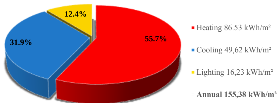
Figure.8. Breakdown of the total annual energy consumption, base case
