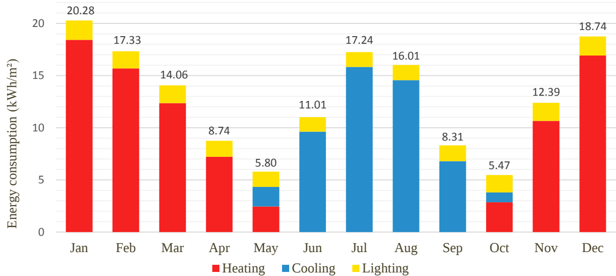
Figure.7. Monthly Baseline Energy Consumption in Bordj Bou Arreridj by End-Use (kWh/m 2 )
