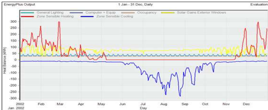
Figure 4. Internal gains and solar infiltration, base case
