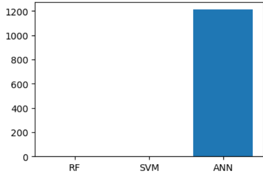
Figure 4: Model Training Time Analysis
